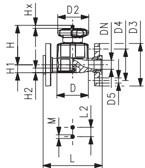
Type 517 Flanged
